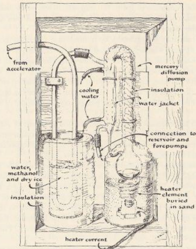
153 Mercury diffusion pump and cold trap for the vacuum system
