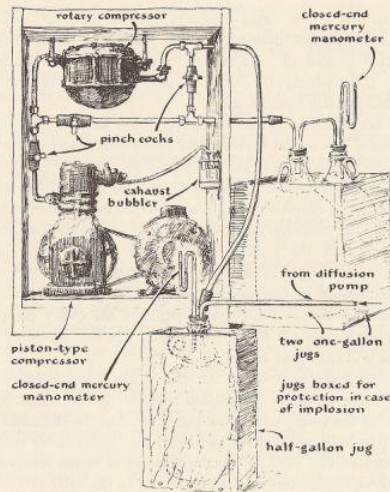
152 "Roughing" pump and reservoirs for vacuum system of the accelerator
